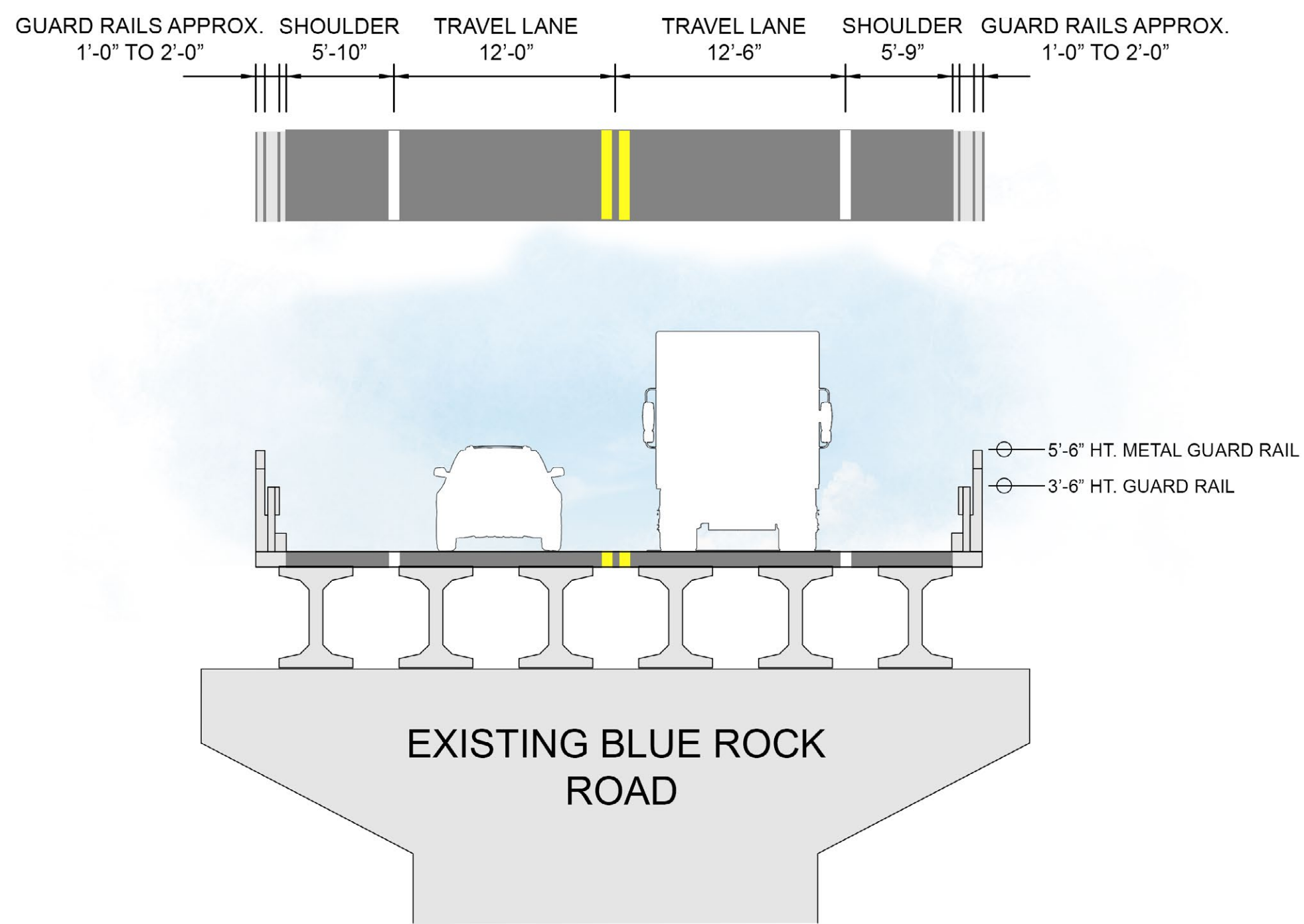
12 EXISTING BLUE ROCK ROAD BRIDGE SECTION NTS
