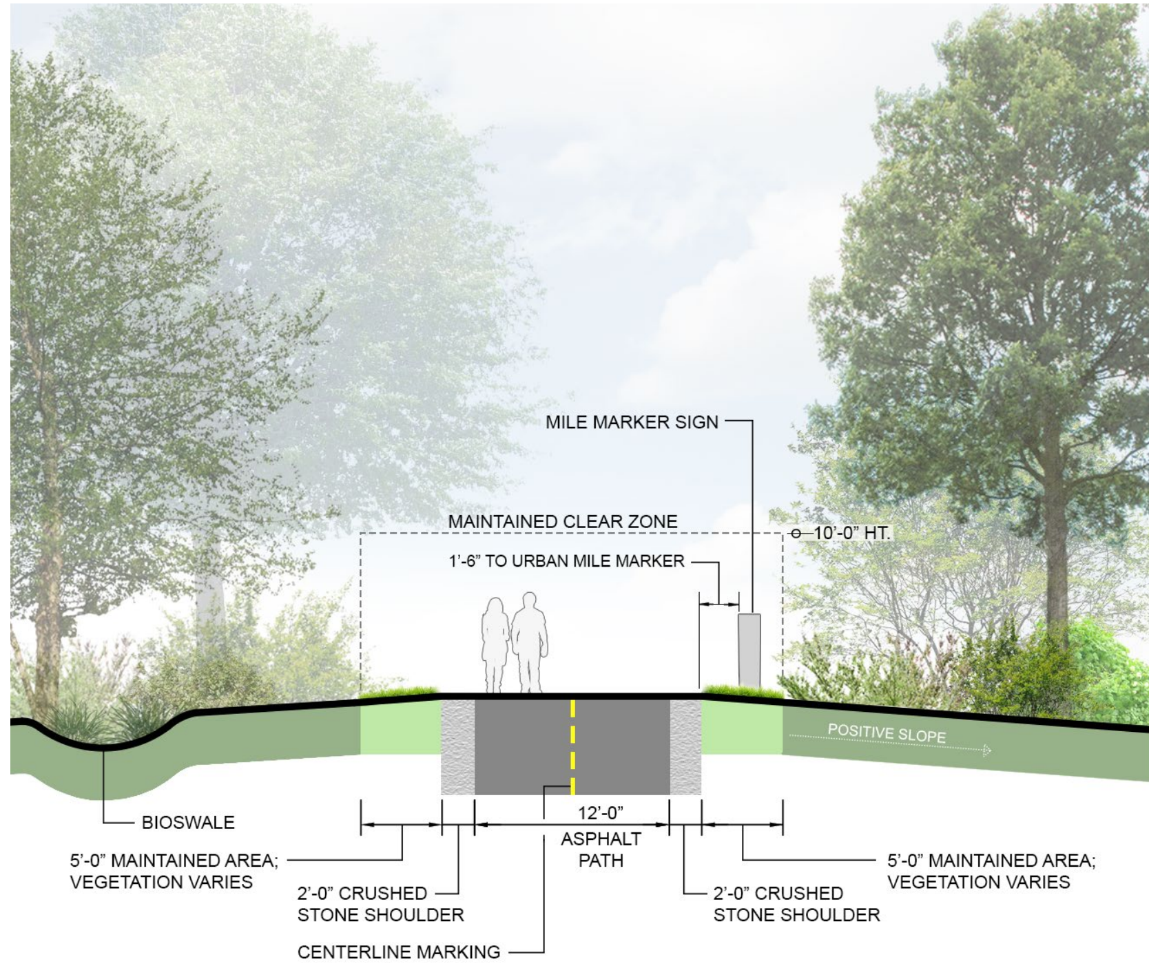
1 TYPICAL SHARED USE TRAIL SECTION
