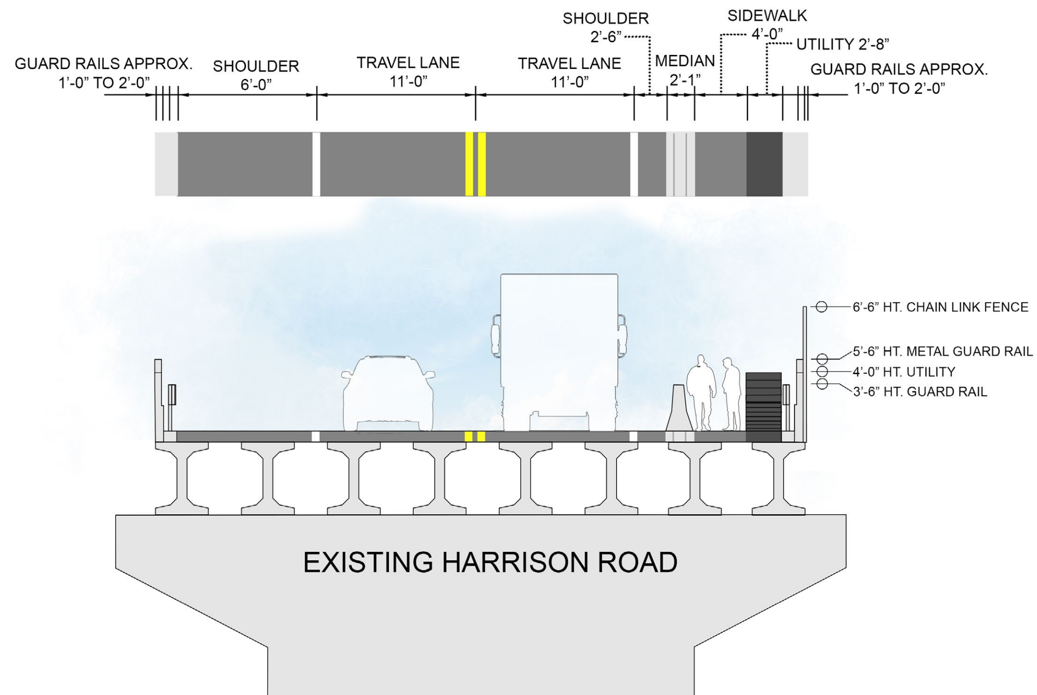
13 EXISTING HARRISON ROAD BRIDGE SECTION NTS
