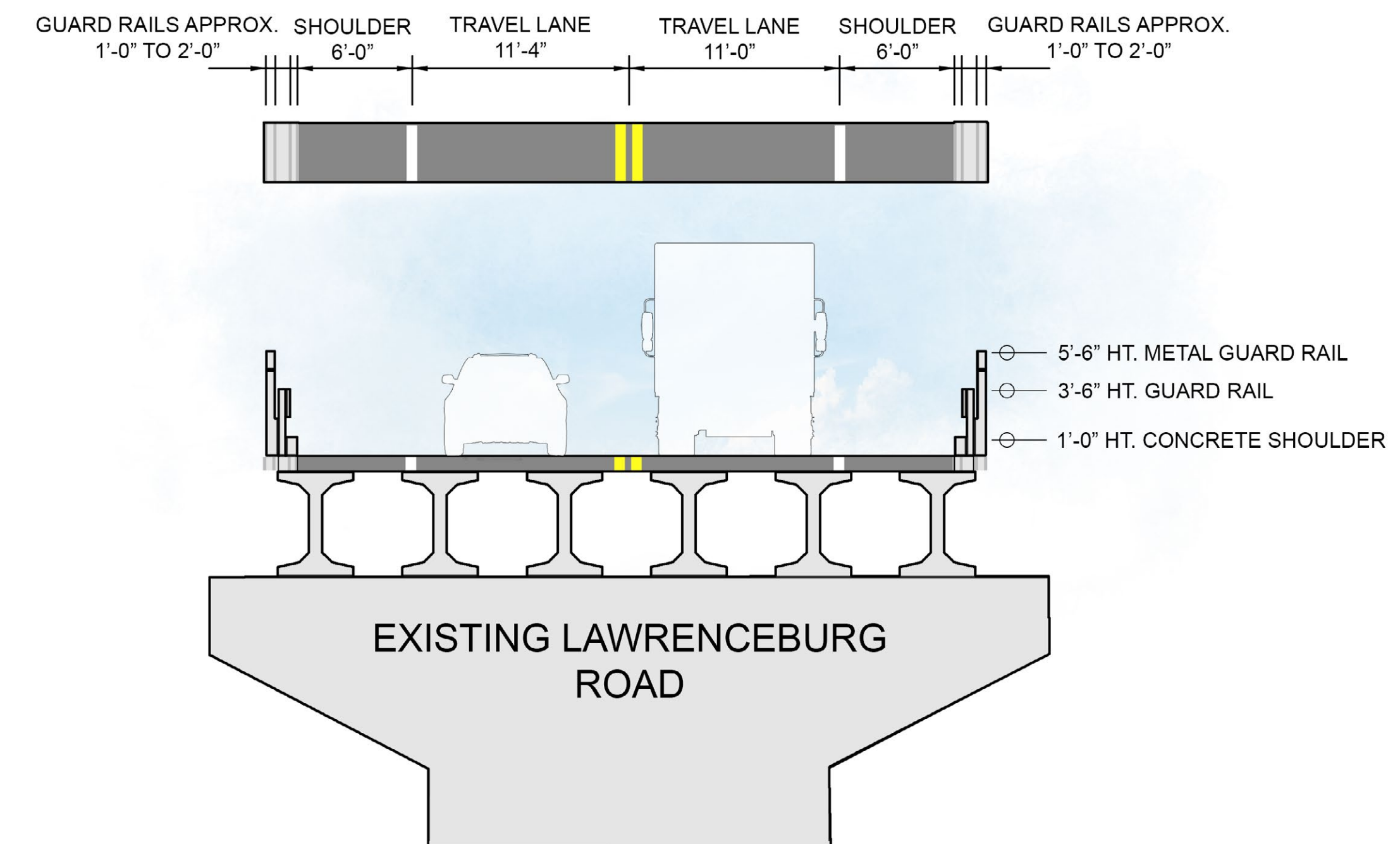
14 EXISTING LAWRENCEBURG ROAD BRIDGE SECTION NTS
