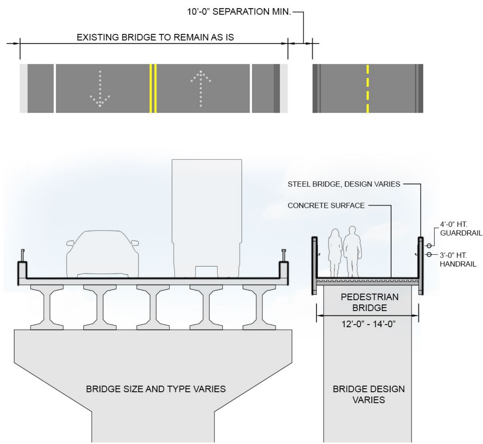
9 TYPICAL PROPOSED DEDICATED PEDESTRIAN BRIDGE NTS
