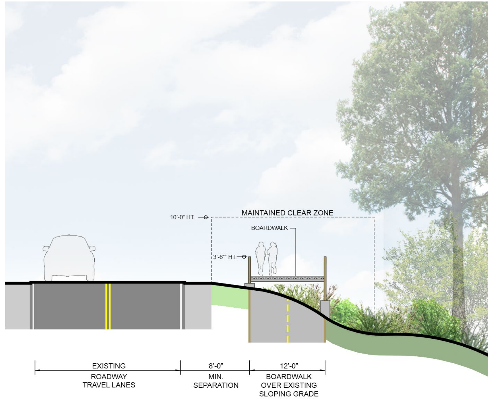
3 TYPICAL BOARDWALK SECTION
