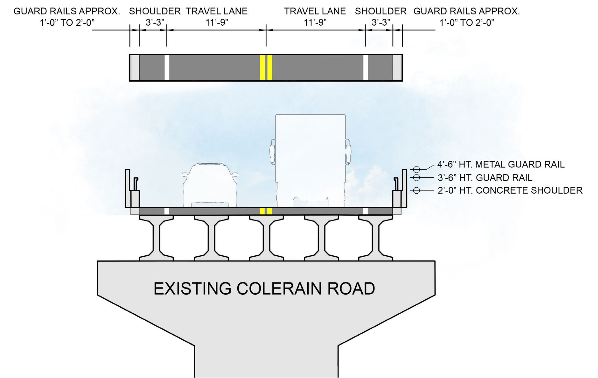
11 EXISTING COLERAIN ROAD BRIDGE SECTION NTS
