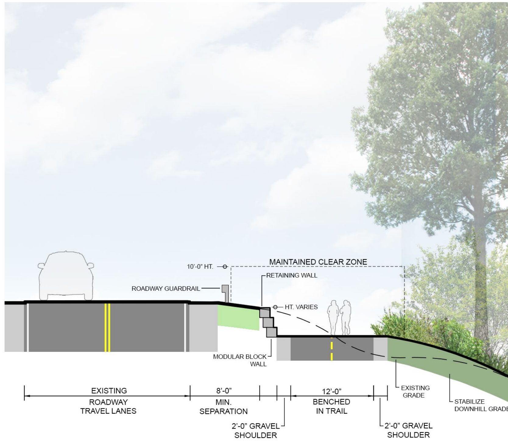
5 TYPICAL BENCHED IN TRAIL SECTION
