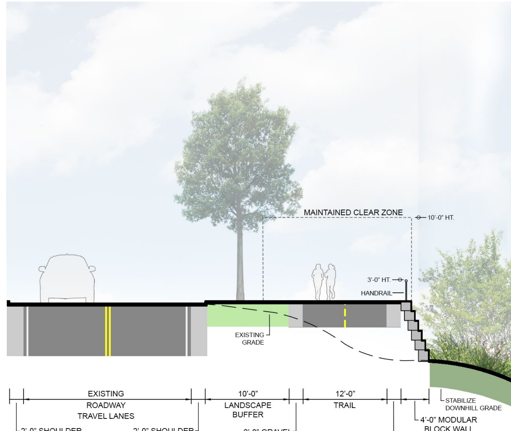
4 TYPICAL RAISED TRAIL SECTION
