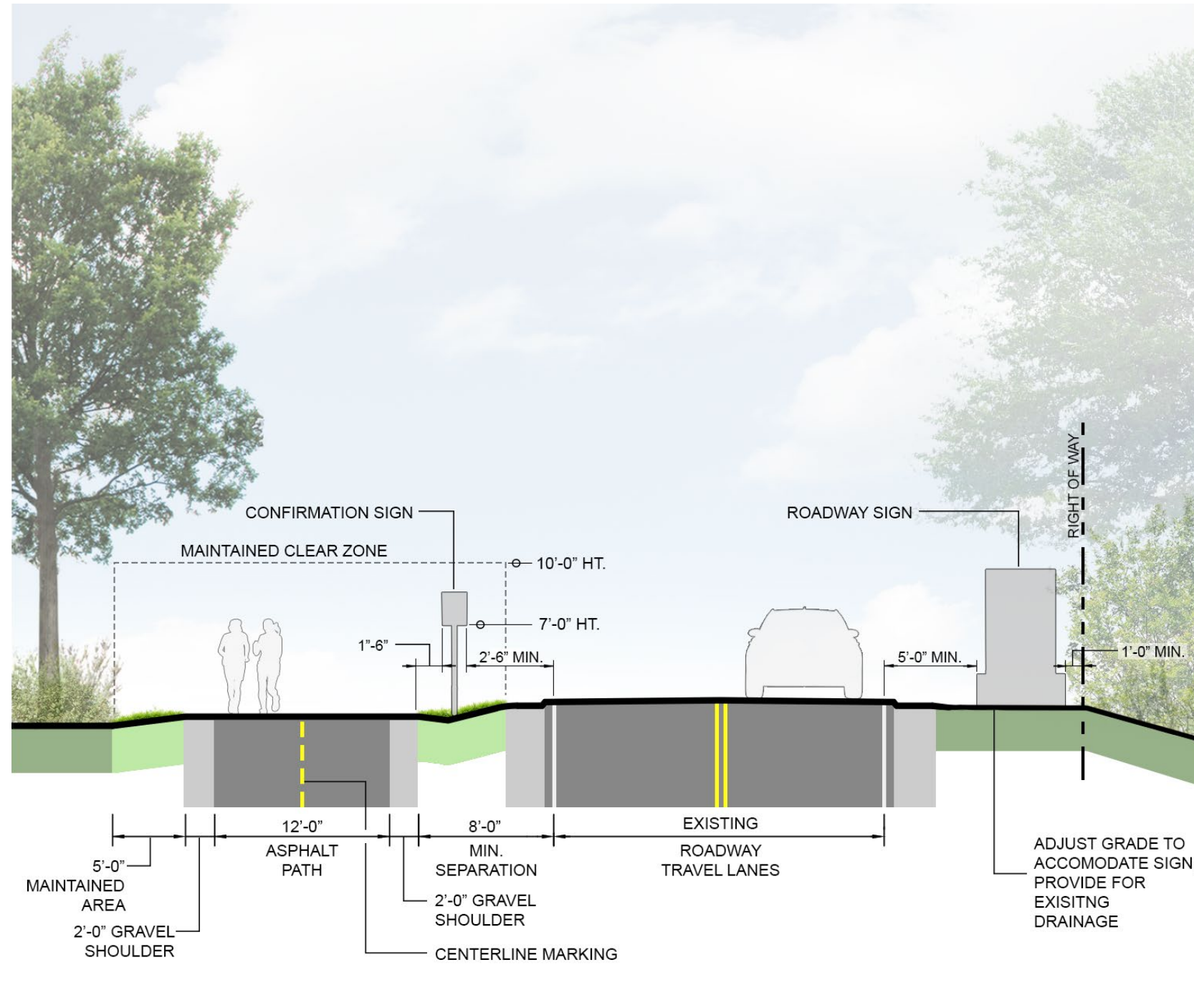
2 TYPICAL SIDEPATH SECTION
