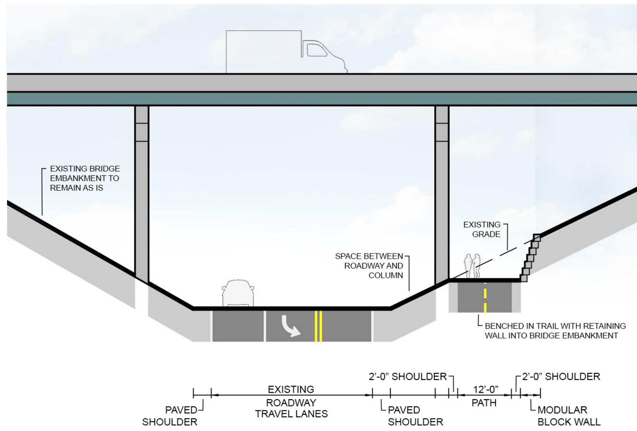
10 TYPICAL UNDERPASS SECTION NTS
