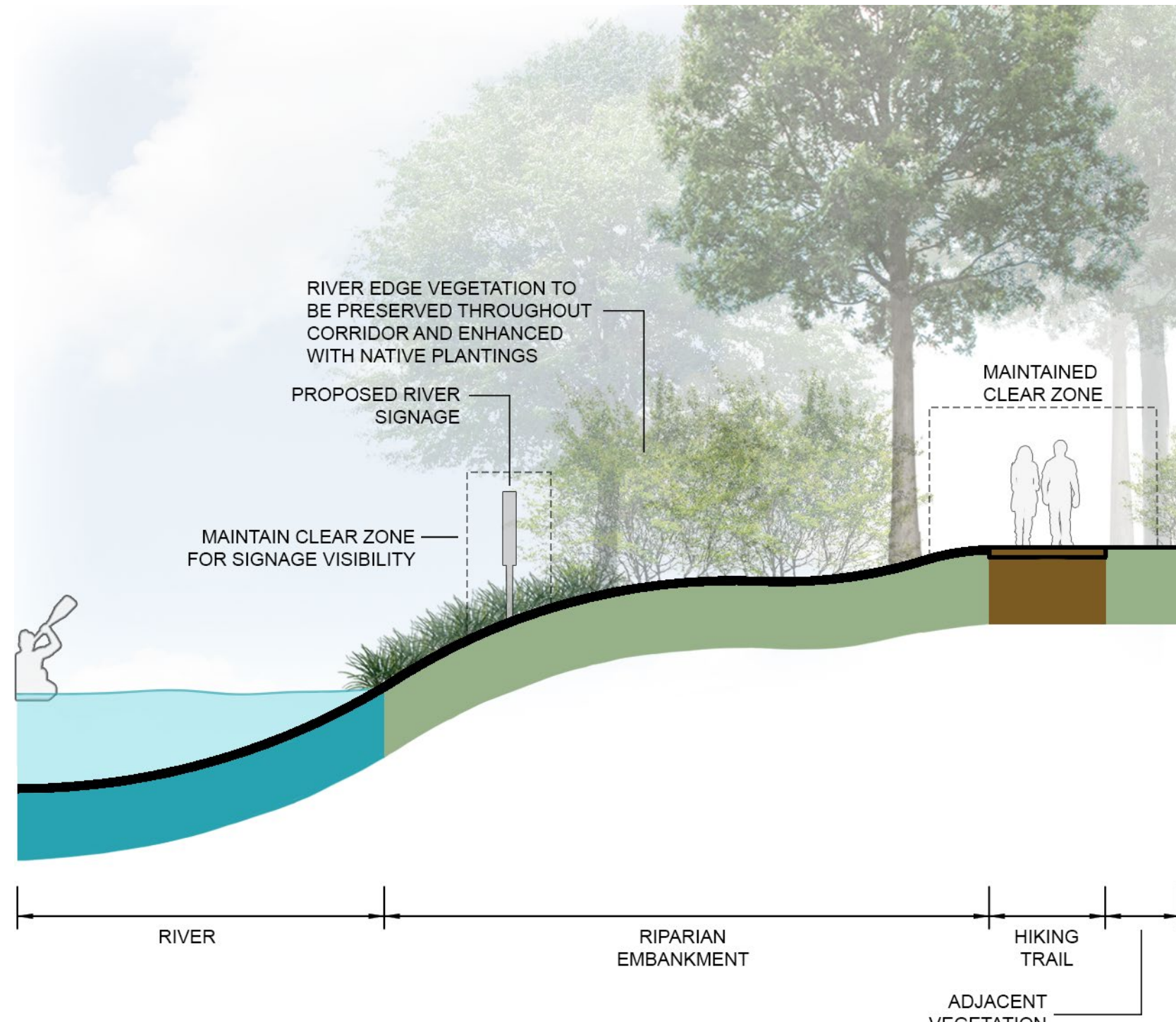
8 TYPICAL HIKING TRAIL SECTION
